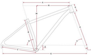
2014 Diamant Mk3 fatbike geometry
