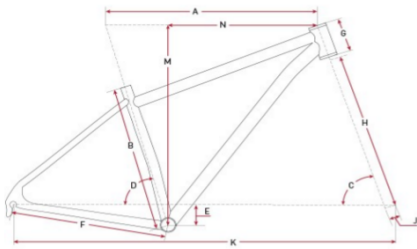
2014 Diamant Mk3 fatbike geometry
